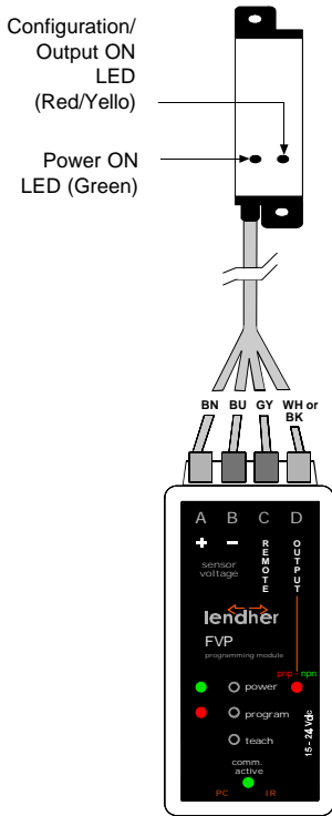
Figure 5. Programming connections using FVP portable module
